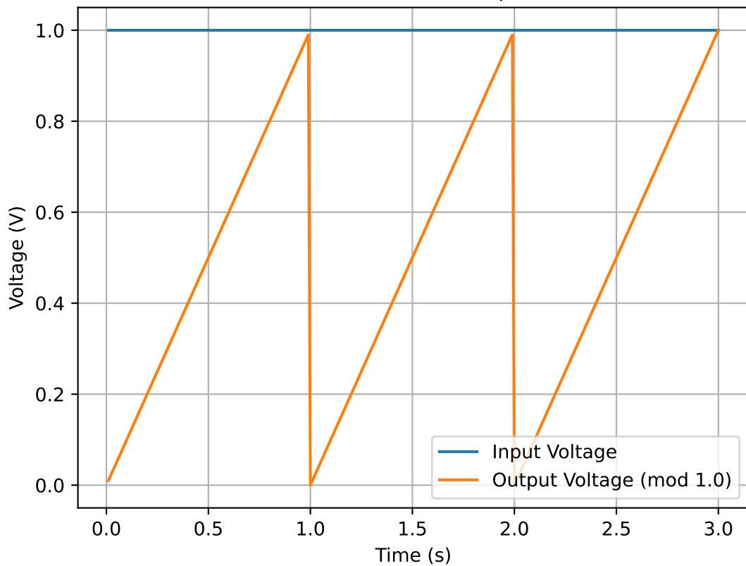
Idtmod Transient Response
